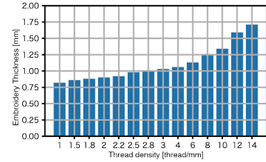
Fig. 5: Embroidery thickness for each stitch density.
