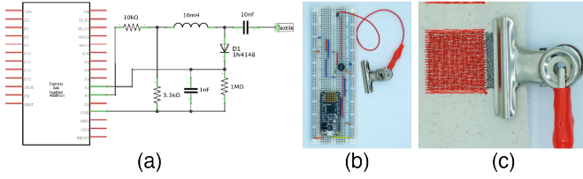
Fig. 3: (a) circuit schematic. (b) We implemented it on a breadboard. (c) Connection of electrodes and circuits by a clip.
