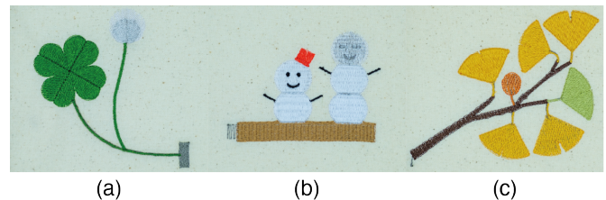
Fig. 1: Examples of touch-sensitive embroideries using our approach: (a) a clover, (b) a snowman, and (c) a ginkgo branch. Our approach adds a non-conductive thread embroidery over an electrode made of conductive threads. By controlling the stitching densities of the upper layer embroidery, developers can achieve different electrical properties at each part of the embroidery. In this manner, it can differentiate touch locations.
