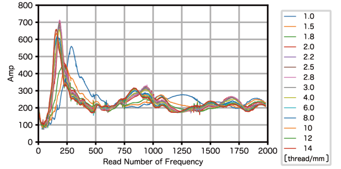
Fig. 4: Impedance during touch for each stitch density of non-conductive threads.
